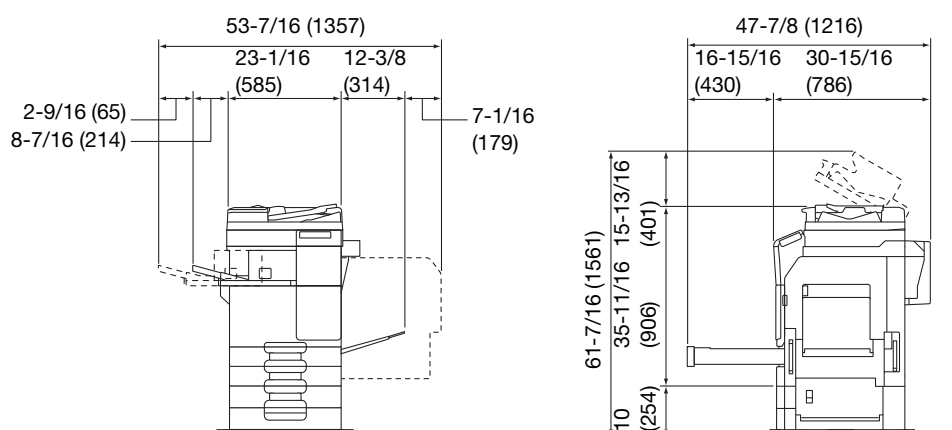
bizhub C287/C227 + DF-628 + PC-214 + MK-603 + MK-602 + FS-533 + PK-519 + MK-748 + CU-101 Unit: inch (mm)
