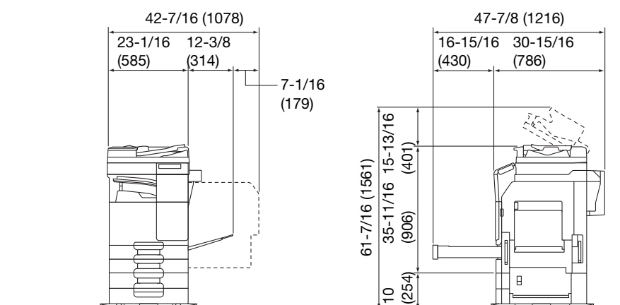
bizhub C287/C227 + DF-628 + PC-214 + MK-603 + JS-506 + MK-748 + CU-101 Unit: inch (mm)
