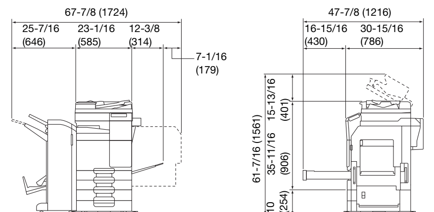
bizhub C287/C227 + DF-628 + PC-214 + MK-603 + RU-514 + FS-534 + SD-511 + MK-748 + CU-101 Unit: inch (mm)
